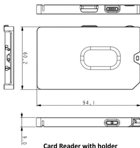
Card Reader with holder
