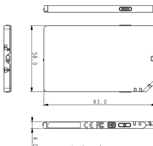
Card Reader
